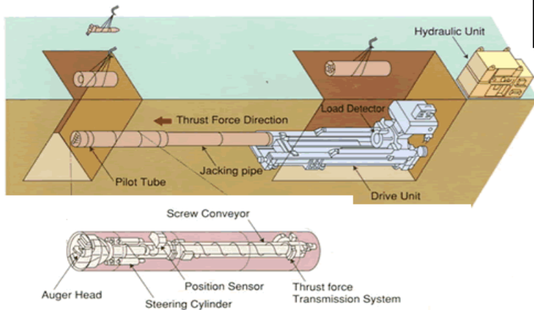
PIPE JACKING
